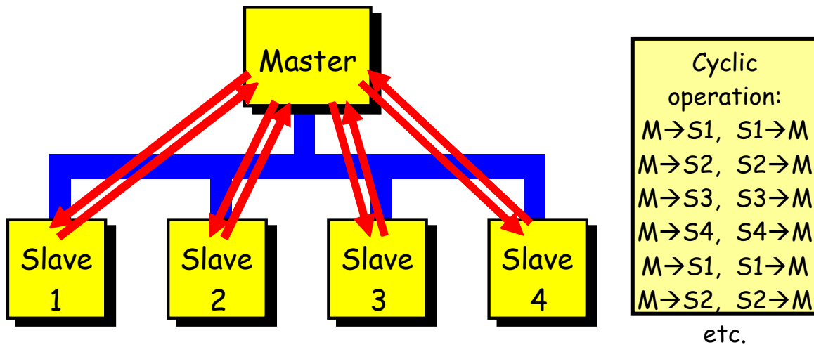
Fig. 1 The Master addresses each slave in turn and gets a reply
