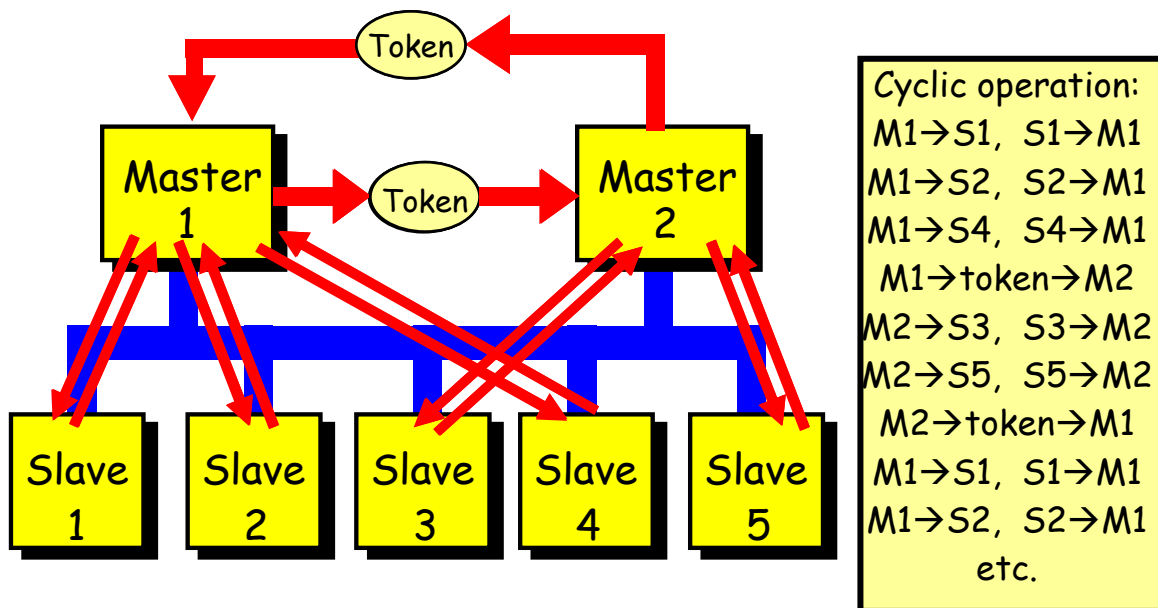
Fig. 2 Master 1 addresses and receives a reply from each of its slaves (1, 2 & 4). The token is passed to Master 2 which then receives a reply from each of its slaves (3 & 5). The token is then passed back to Master 1,
